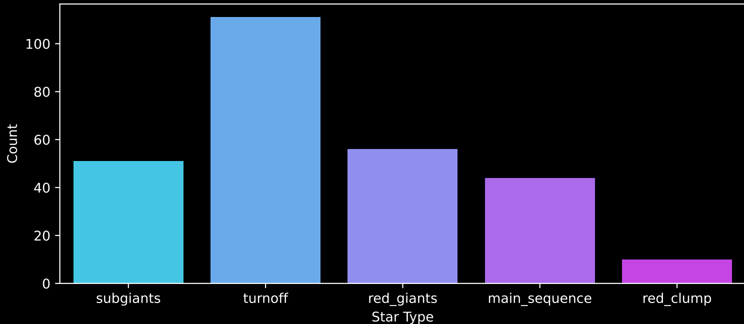
GALAH DR4 Field: [9158] Count plot of Star Type
