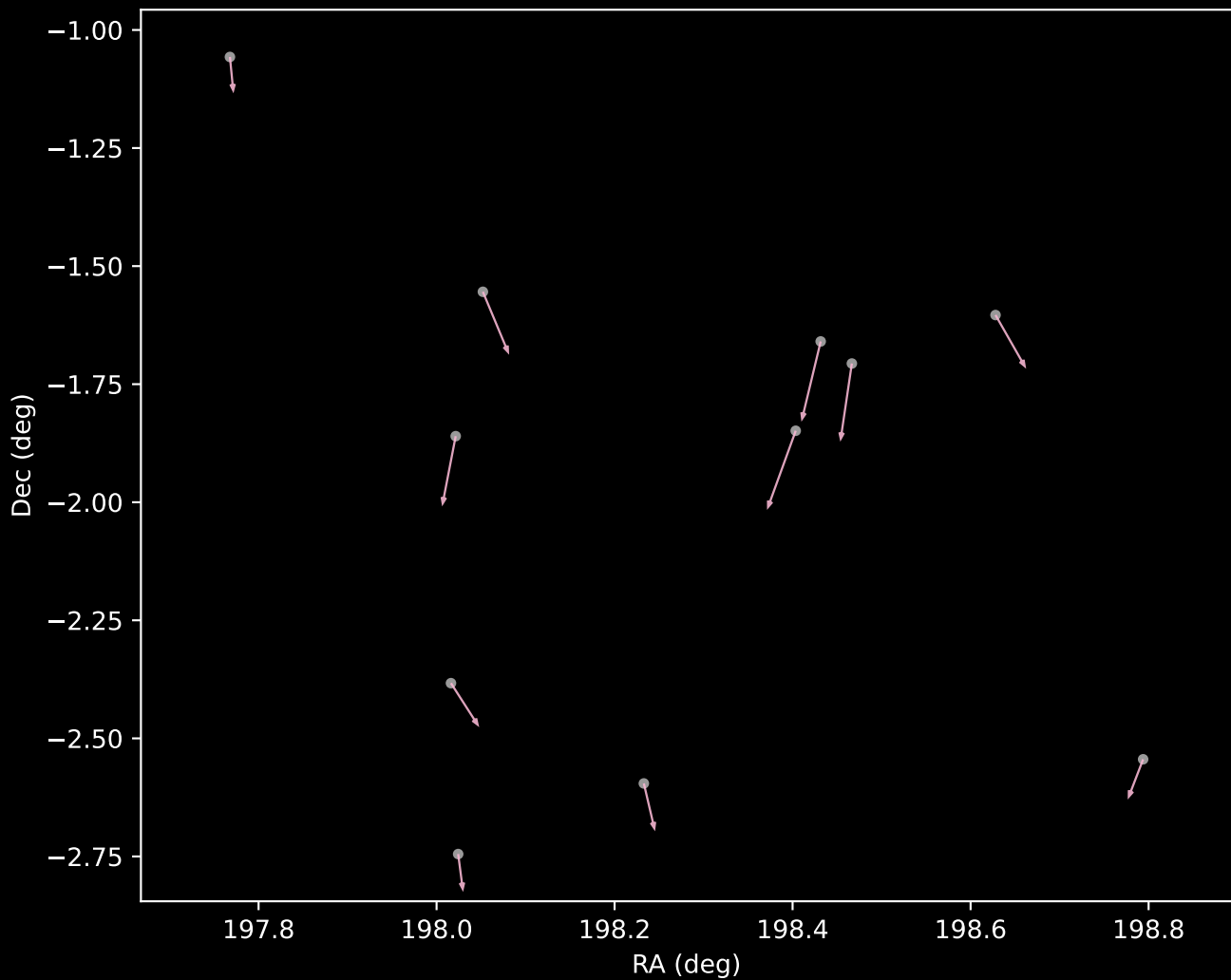
GALAH DR4 Cluster 13 Proper Motion Vectors (n=11)
