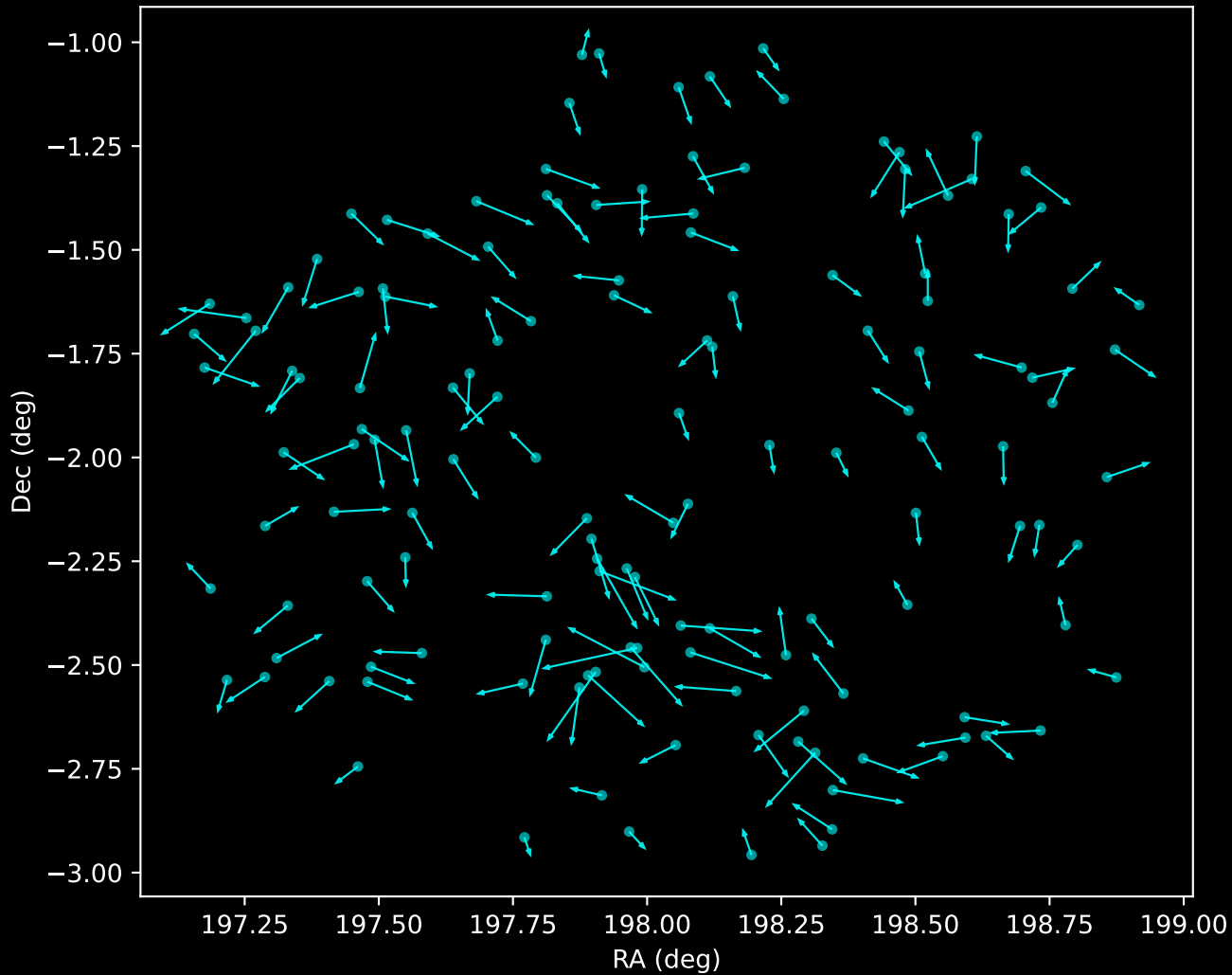
GALAH DR4 Noise Stream Proper Motion Vectors (n=142)
