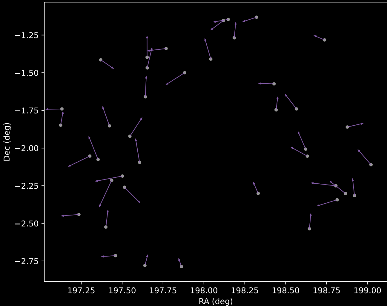
GALAH DR4 Cluster 8 Proper Motion Vectors (n=40)
