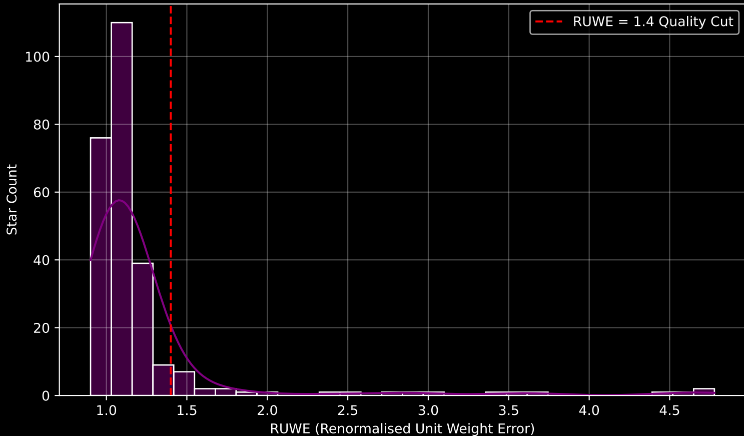
GALAH DR4 Field [9158] RUWE Distribution (n= 259)
